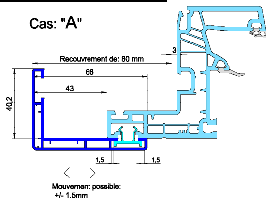
Habillage Compensation ABAQ20
