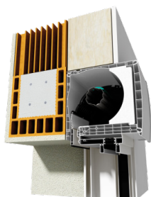
BLOC-BAIE THERMOBLOC
